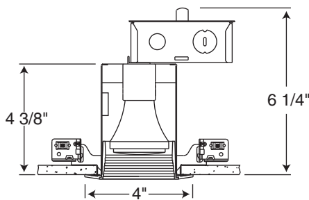
3 1/4" sq. Ceiling Cutout
